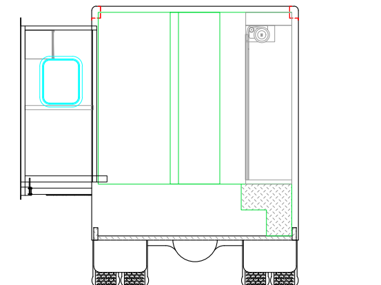
FRONT WALK-IN CROSS-SECTION
