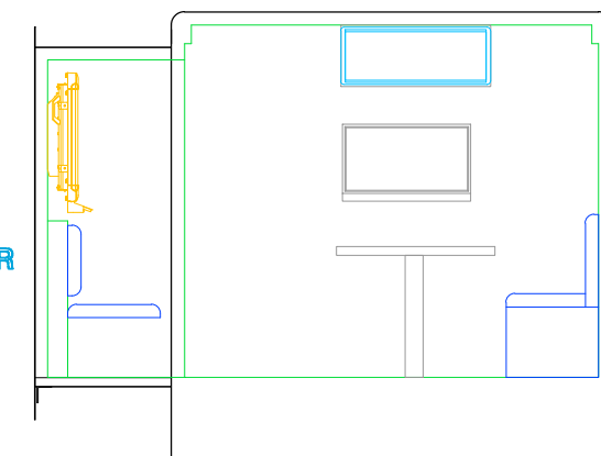
REAR VIEW OF BODY CROSS-SECTION
